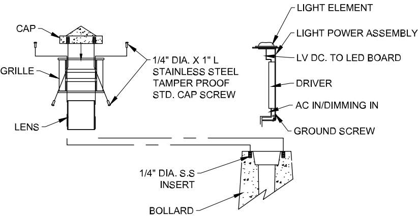
BOLLARD HEAD & ELECTRICAL DETAIL
