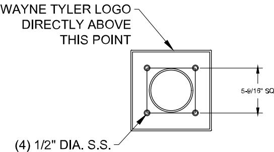
ANCHOR BOLT PATTERN
