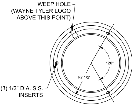
ANCHOR BOLT PATTERN
