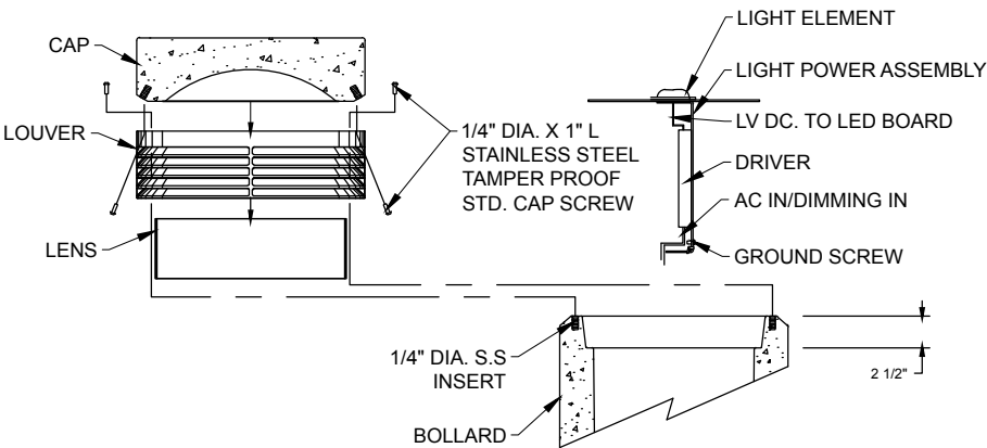
BOLLARD HEAD & ELECTRICAL DETAIL
