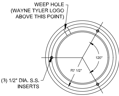
ANCHOR BOLT PATTERN
