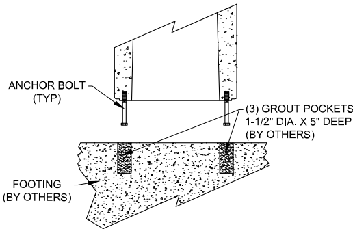
BOLLARD MOUNT DETAIL
