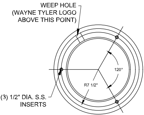
ANCHOR BOLT PATTERN
