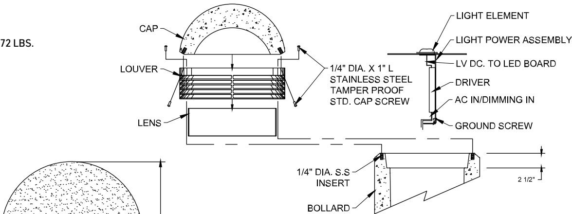
BOLLARD HEAD & ELECTRICAL DETAIL
