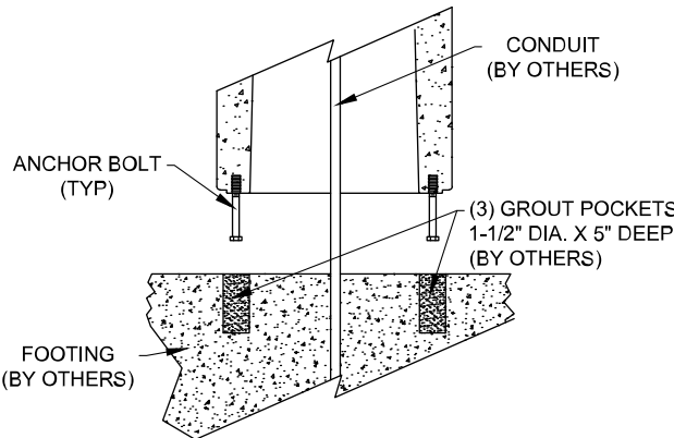
BOLLARD MOUNT DETAIL
