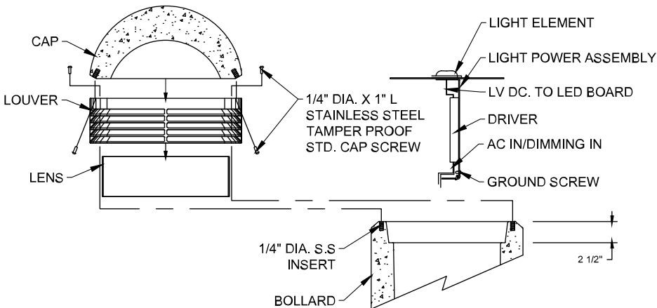
BOLLARD HEAD & ELECTRICAL DETAIL
