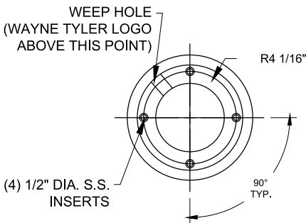
ANCHOR BOLT PATTERN
