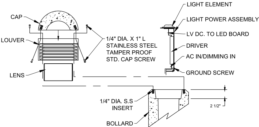
BOLLARD HEAD & ELECTRICAL DETAIL
