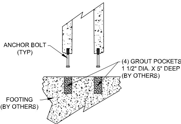
BOLLARD MOUNT DETAIL
