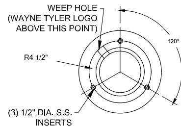
ANCHOR BOLT PATTERN
