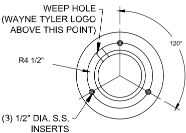
ANCHOR BOLT PATTERN
