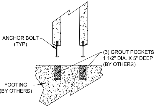
BOLLARD MOUNT DETAIL
