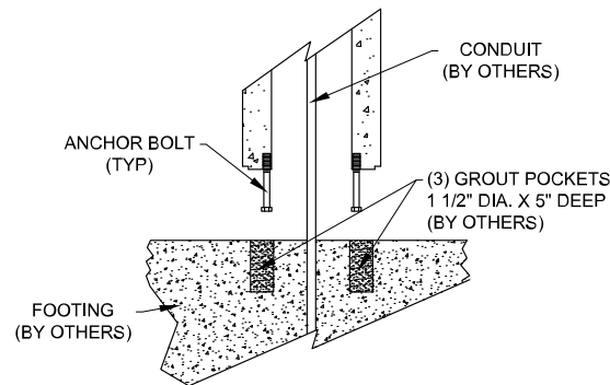
BOLLARD MOUNT DETAIL
