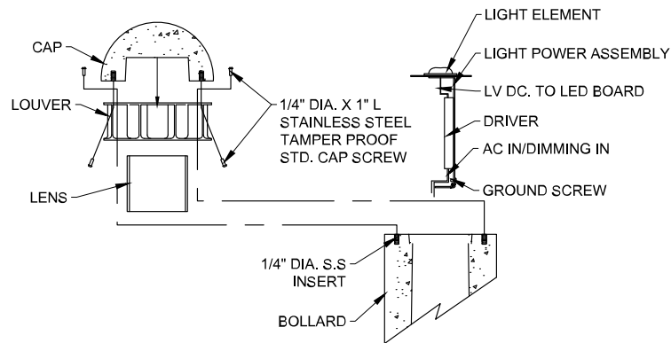
BOLLARD HEAD & ELECTRICAL DETAIL
