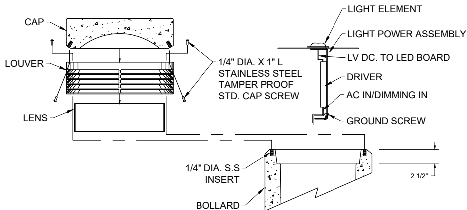
BOLLARD HEAD & ELECTRICAL DETAIL
