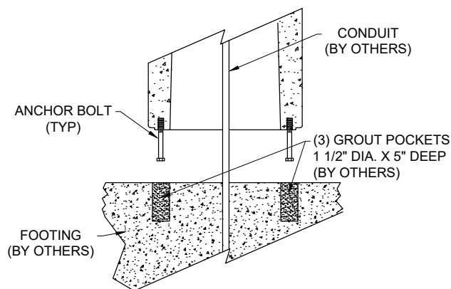
BOLLARD MOUNT DETAIL
