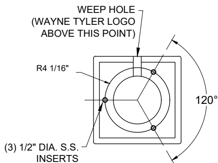
ANCHOR BOLT PATTERN
