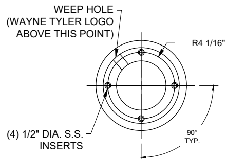
ANCHOR BOLT PATTERN
