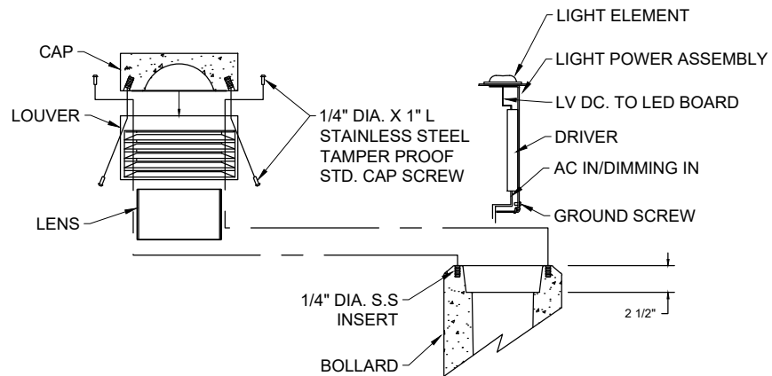
BOLLARD HEAD & ELECTRICAL DETAIL
