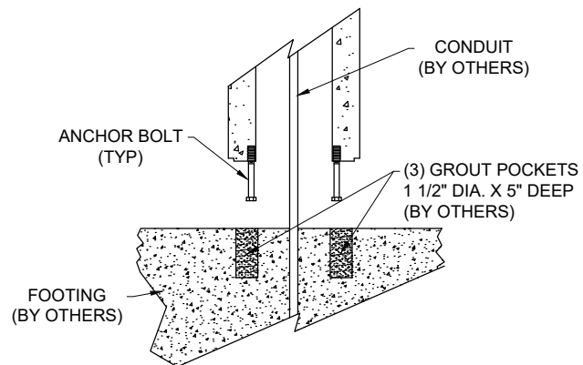
BOLLARD MOUNT DETAIL
