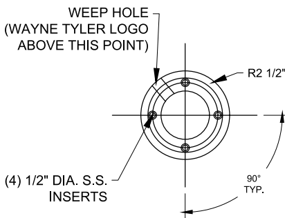
ANCHOR BOLT PATTERN
