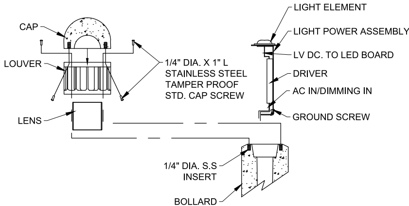
BOLLARD HEAD & ELECTRICAL DETAIL
