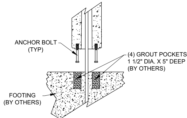
BOLLARD MOUNT DETAIL
