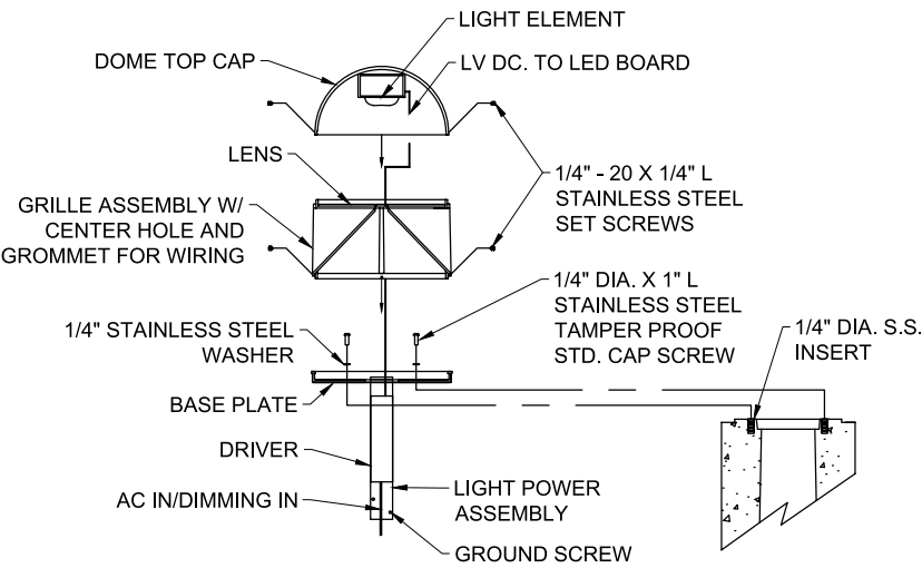
BOLLARD HEAD & ELECTRICAL DETAIL
