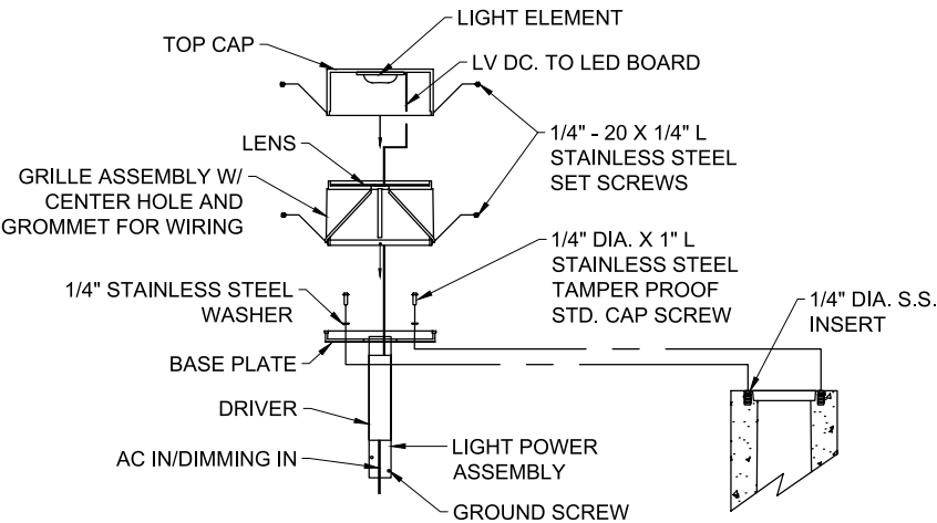
BOLLARD HEAD & ELECTRICAL DETAIL
