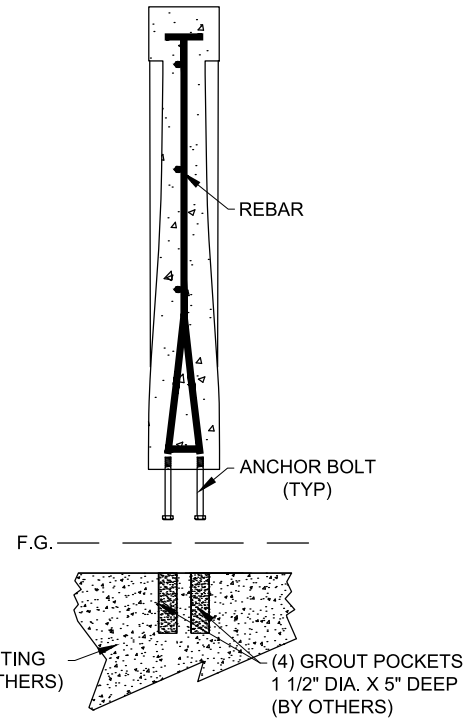
SECTION DETAIL
