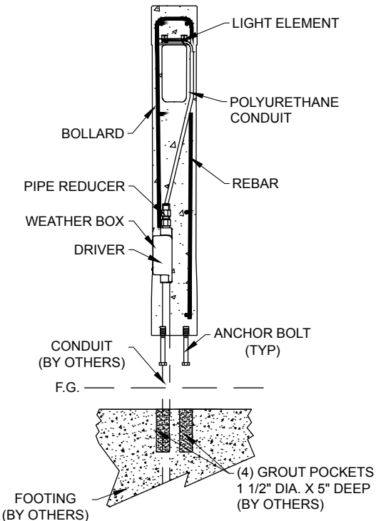
SECTION DETAIL
