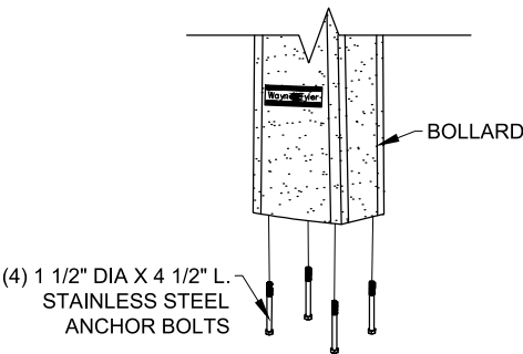
MOUNTING DETAIL
