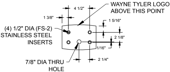
ANCHOR BOLT PATTERN
