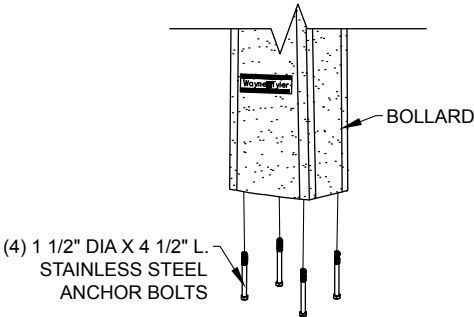
MOUNTING DETAIL
