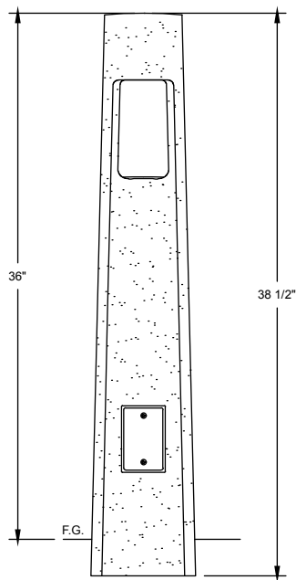
REAR ELEVATION
