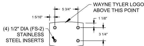
MOUNTING DETAIL
