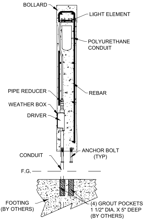
SECTION DETAIL
