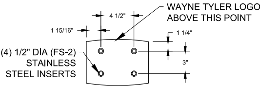
ANCHOR BOLT PATTERN
