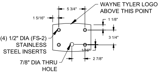
ANCHOR BOLT PATTERN
