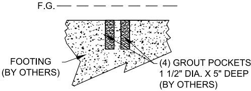
SECTION DETAIL
