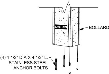
MOUNTING DETAIL
