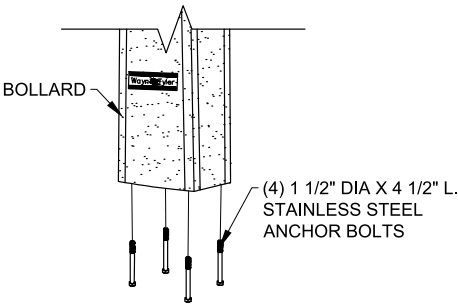
MOUNTING DETAIL
