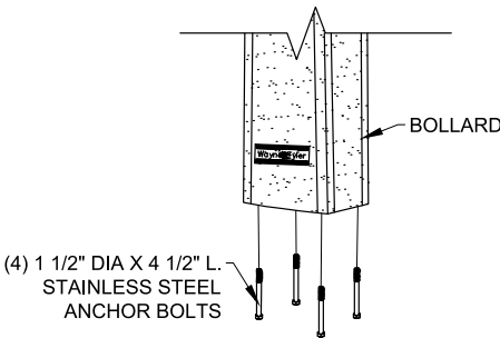
MOUNTING DETAIL
