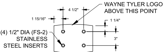
ANCHOR BOLT PATTERN
