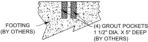
SECTION DETAIL
