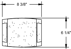
PLAN VIEW
