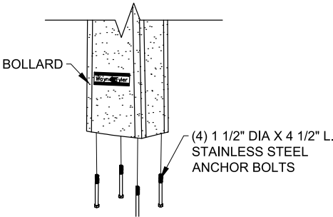
MOUNTING DETAIL
