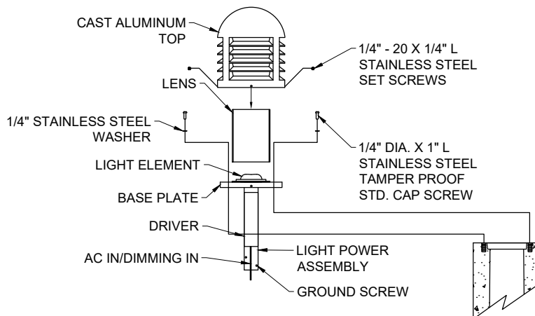
BOLLARD HEAD & ELECTRICAL DETAIL
