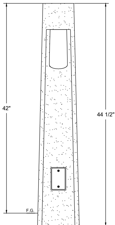
REAR ELEVATION
