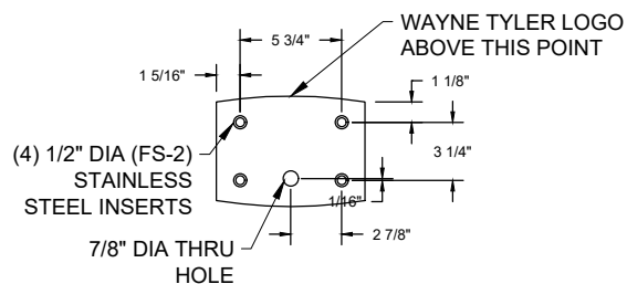
ANCHOR BOLT PATTERN
