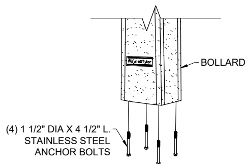
MOUNTING DETAIL
