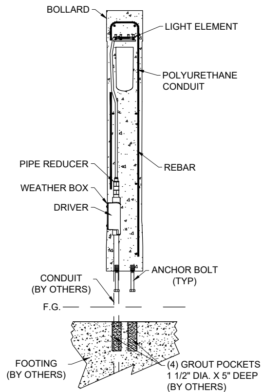
SECTION DETAIL
