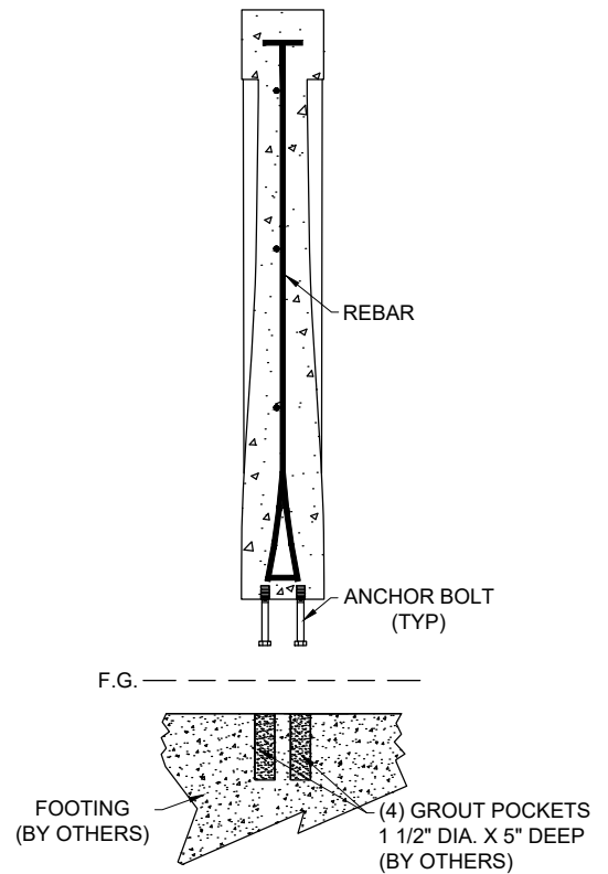
SECTION DETAIL
