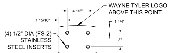
MOUNTING DETAIL
