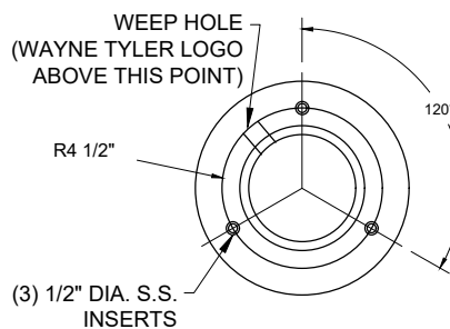
ANCHOR BOLT PATTERN
