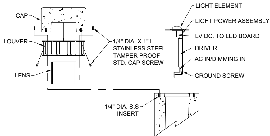
BOLLARD HEAD & ELECTRICAL DETAIL
