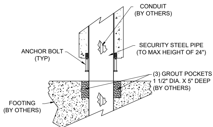
BOLLARD MOUNT DETAIL
